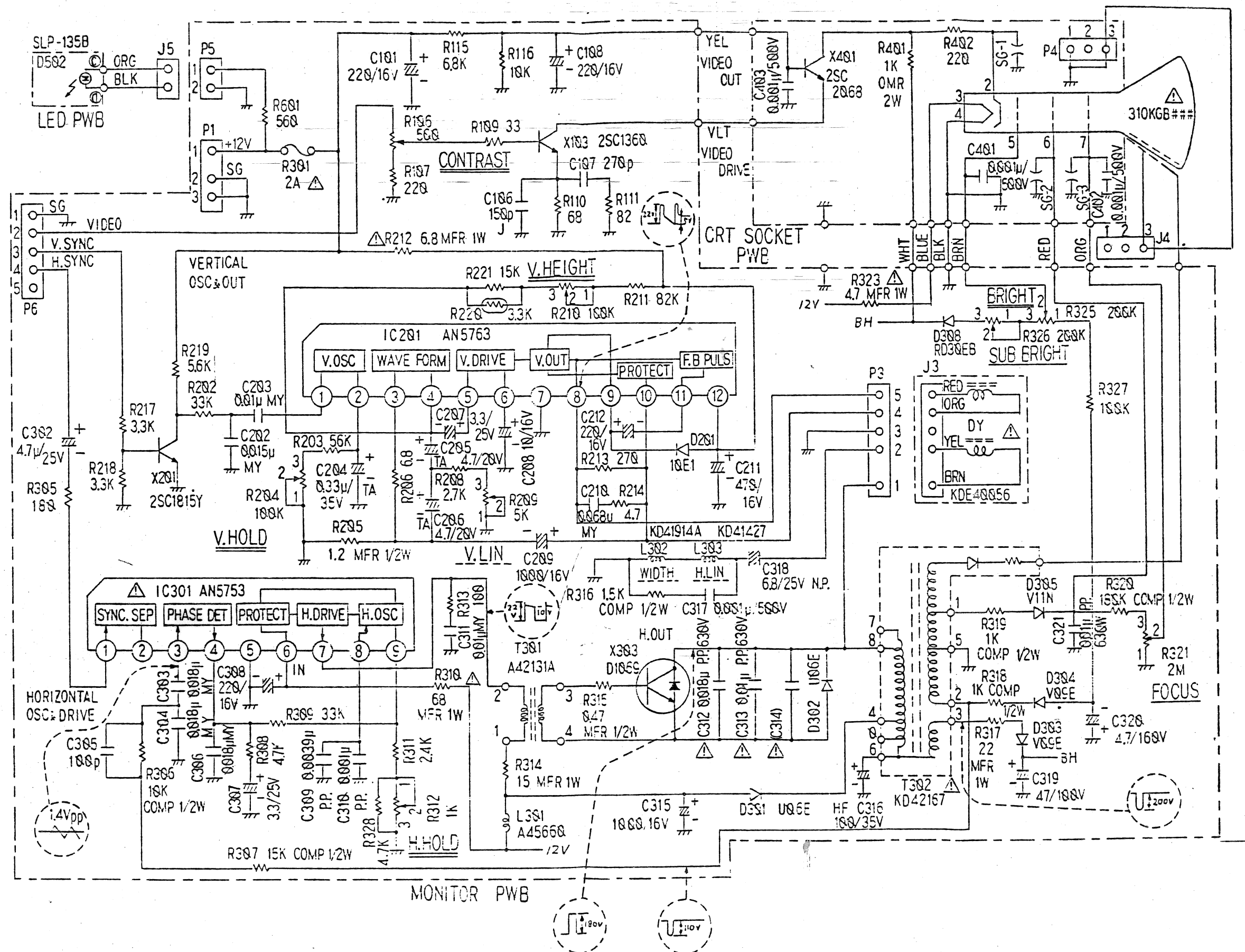
FIG. 10-3 VG-920 MONITOR PWB
