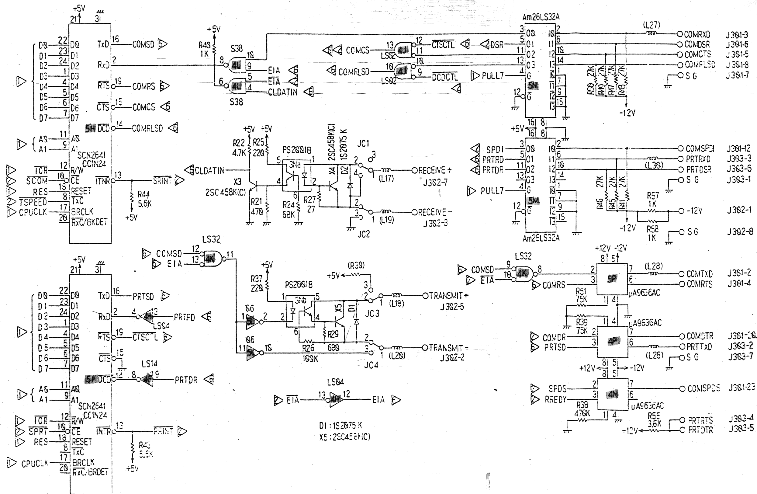
FIG. 10-2 VG-920 LOGIC PWB 6/6
