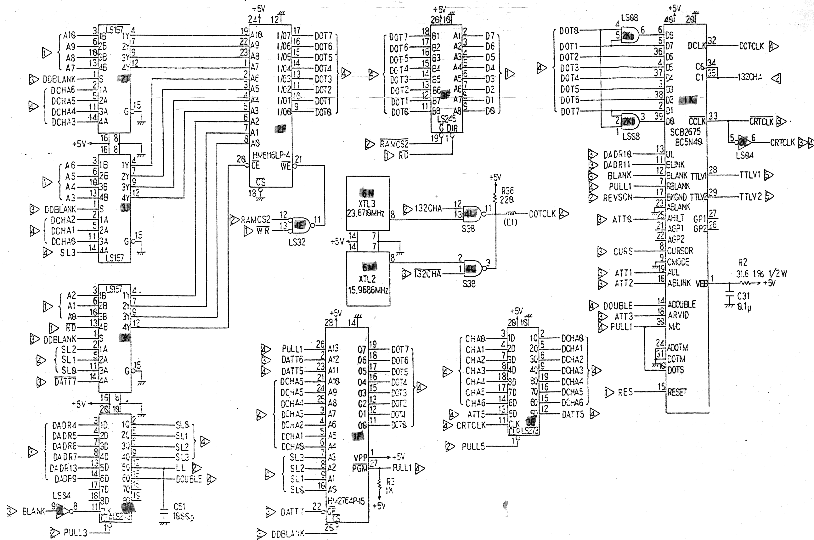
FIG. 10-2 VG-920 LOGIC PWB 4/6
