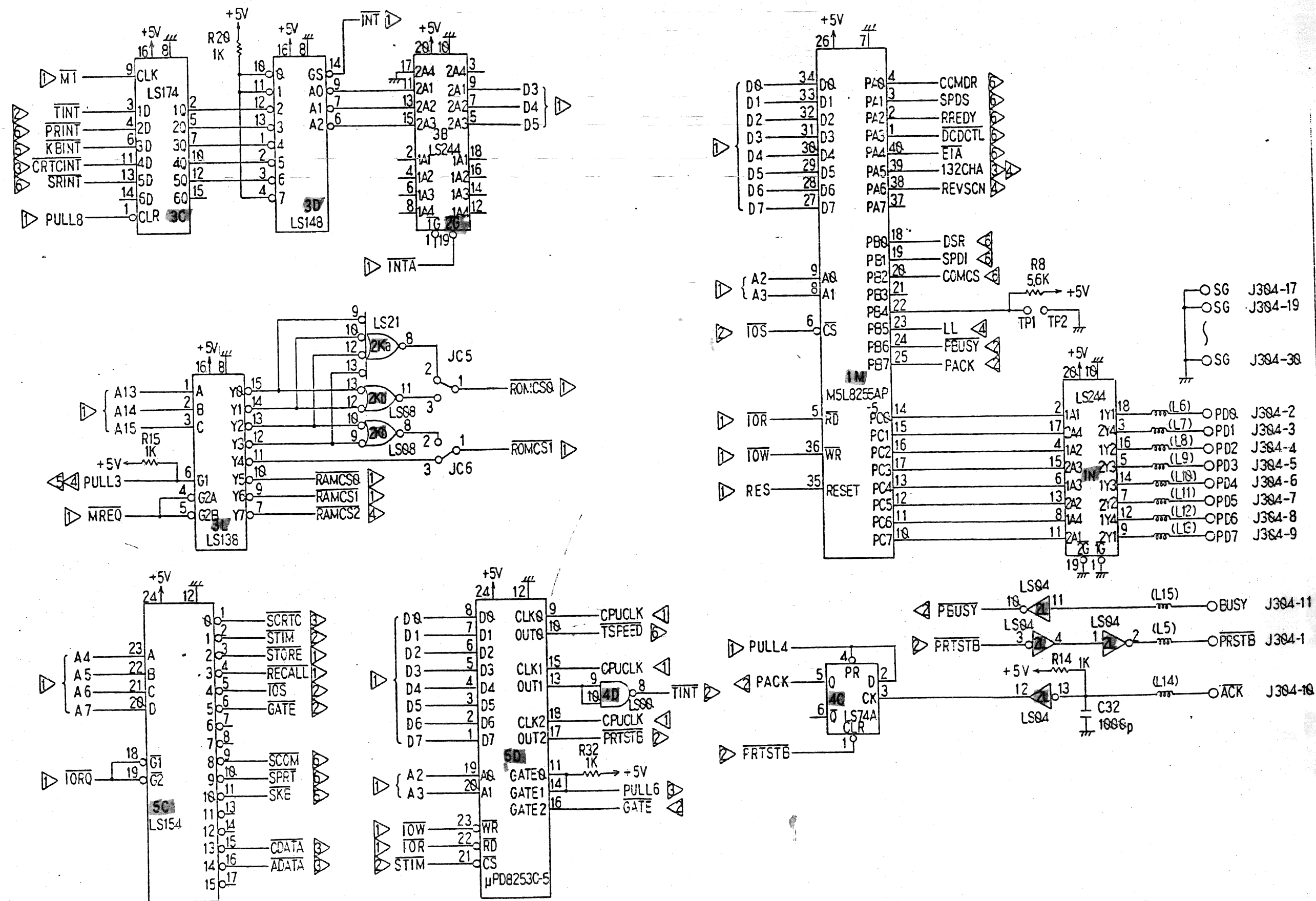
FIG. 10-2 VG-920 LOGIC PWB 2/6
