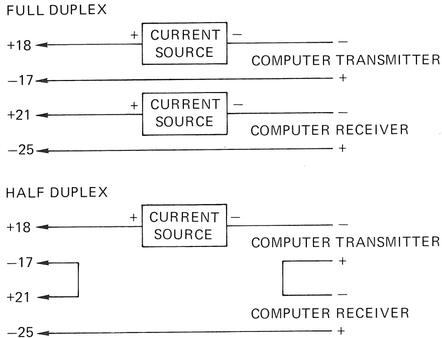
Figure 5-2 Current Loop Connections
