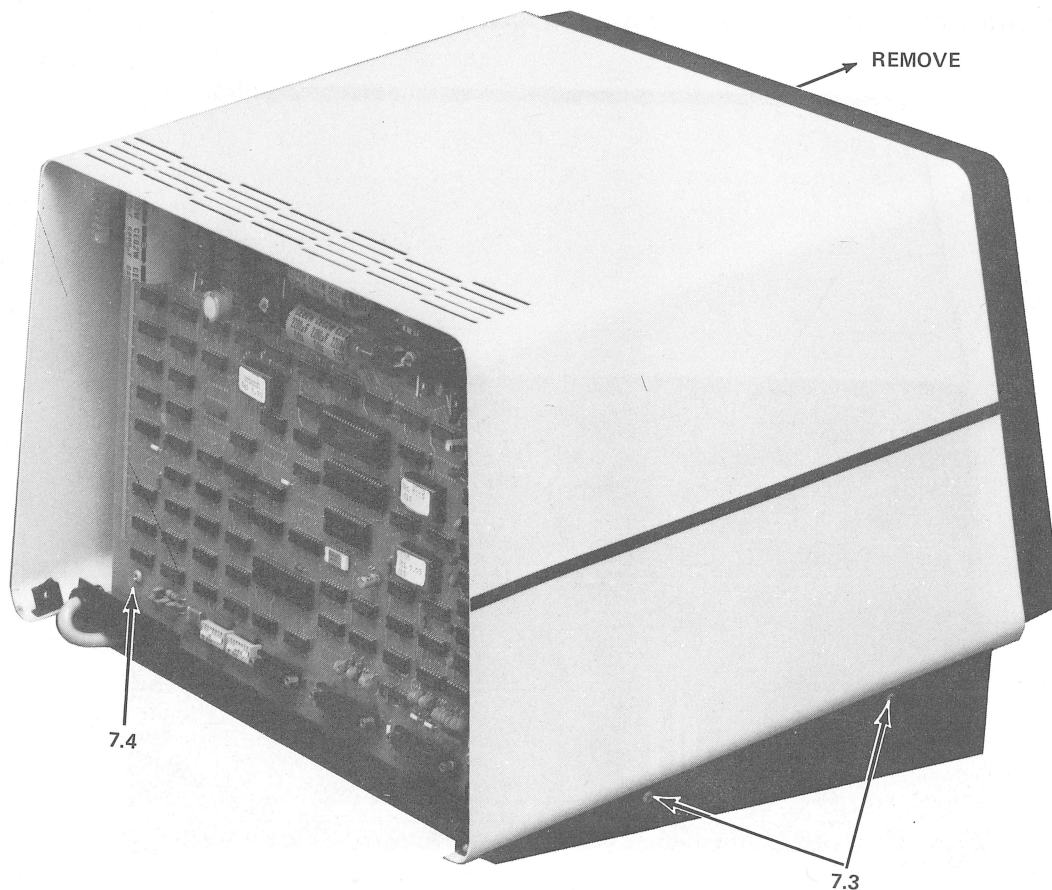
Figure 7-2 Top Cover Removal
