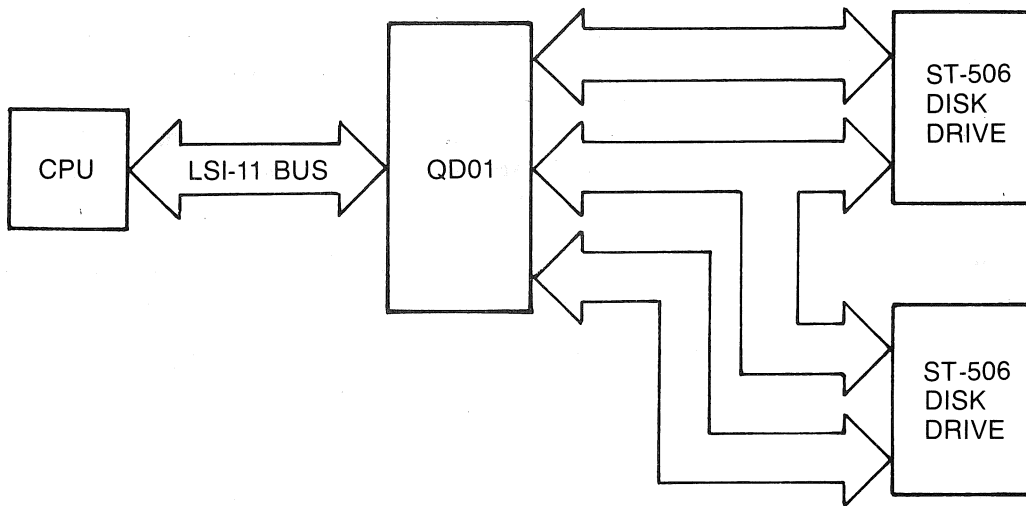
Figure 1-1. QD01/D Subsystem Configuration
