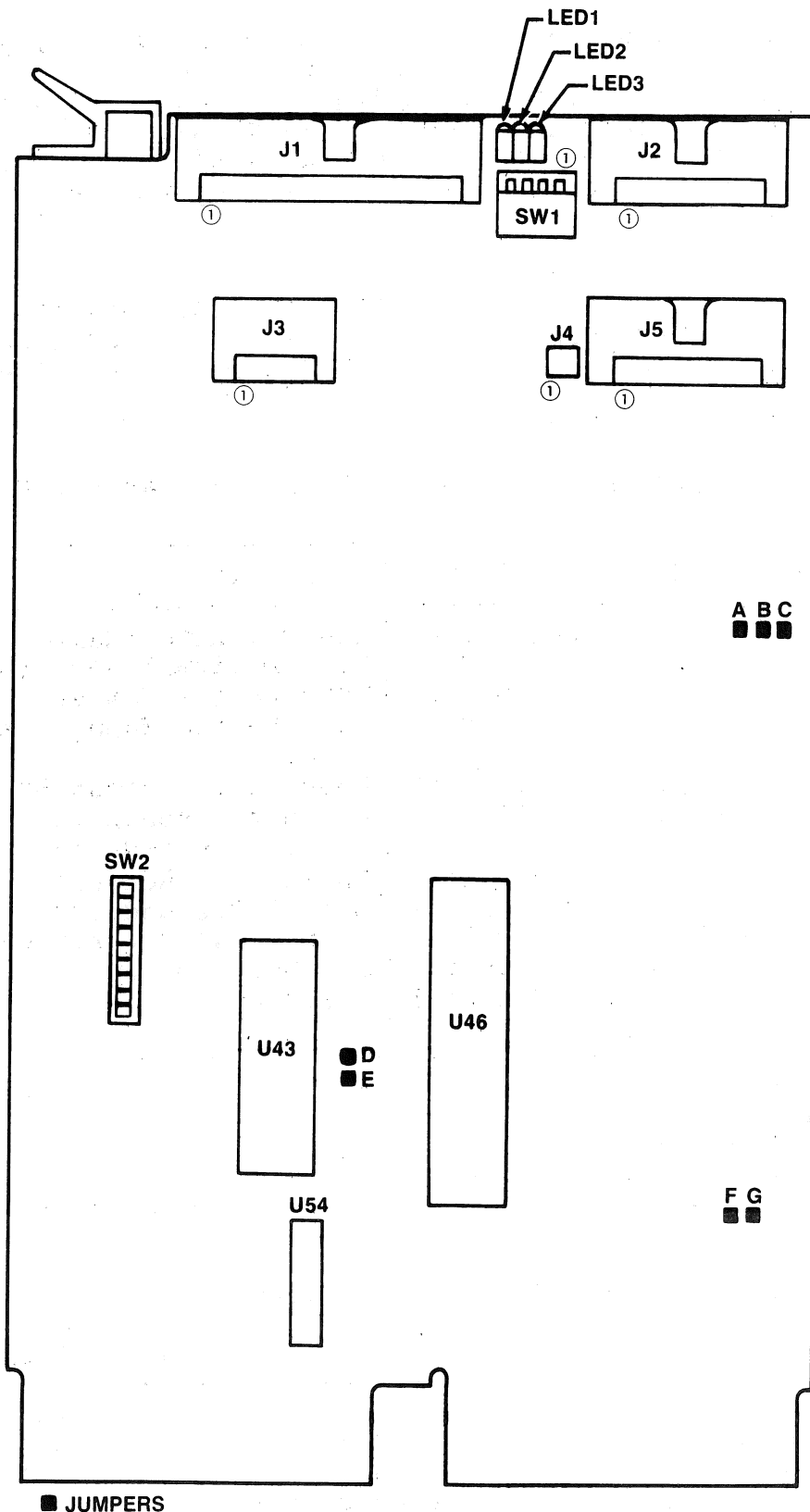
Figure 4-3. QD01/D Disk Controller Assembly
