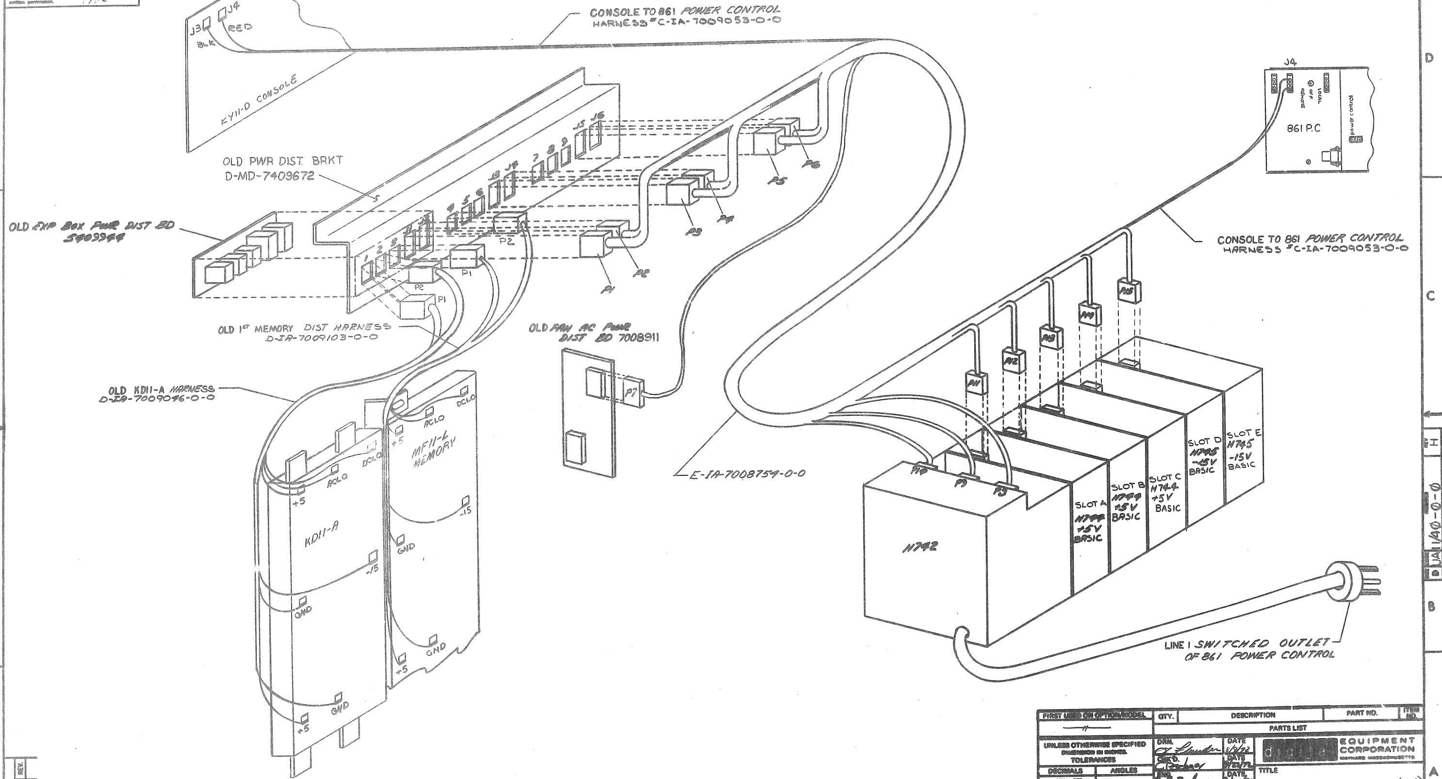
OLD PWR DISTRIBUTION VERSION FOR SYSTEM SERIAL NUMBERS 5999 AND LOWER.
