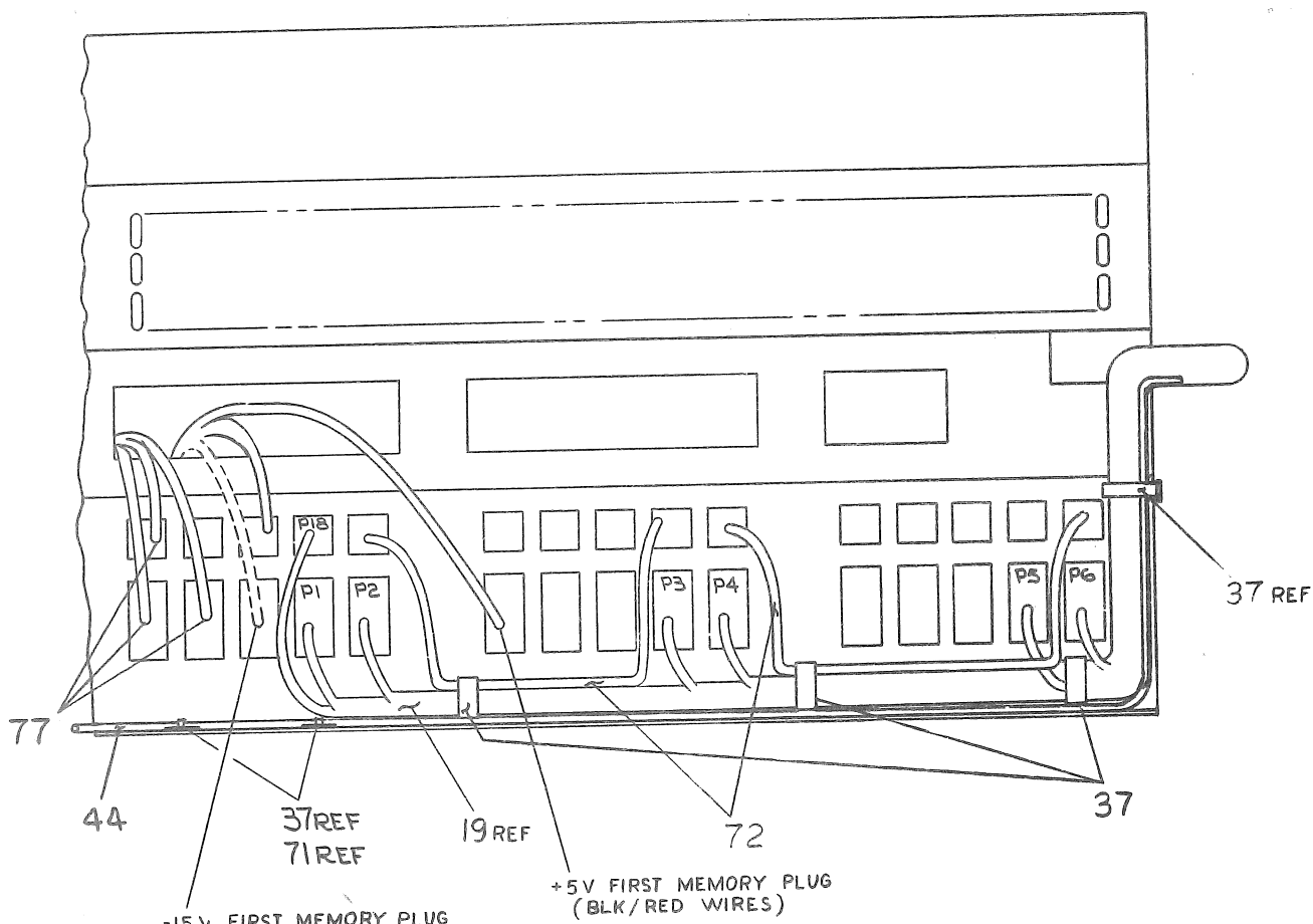
VIEW F-F (ENLARGED VIEW)
