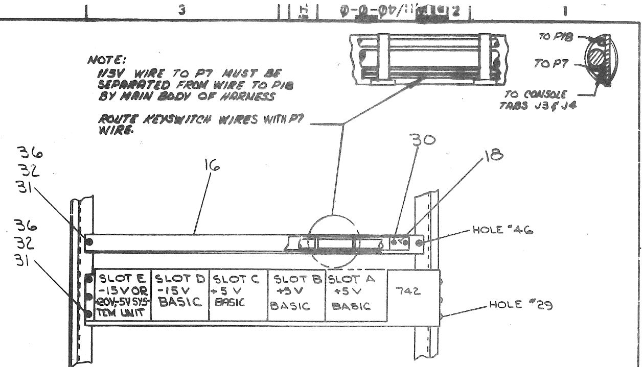
VIEW B-B
