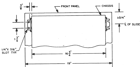
Figure 10.4 Rear View of Mounting Hardware
