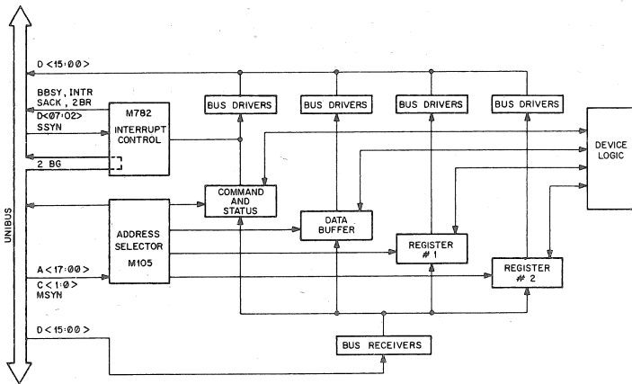
Figure 9.1 Typical Peripheral Device Interface
