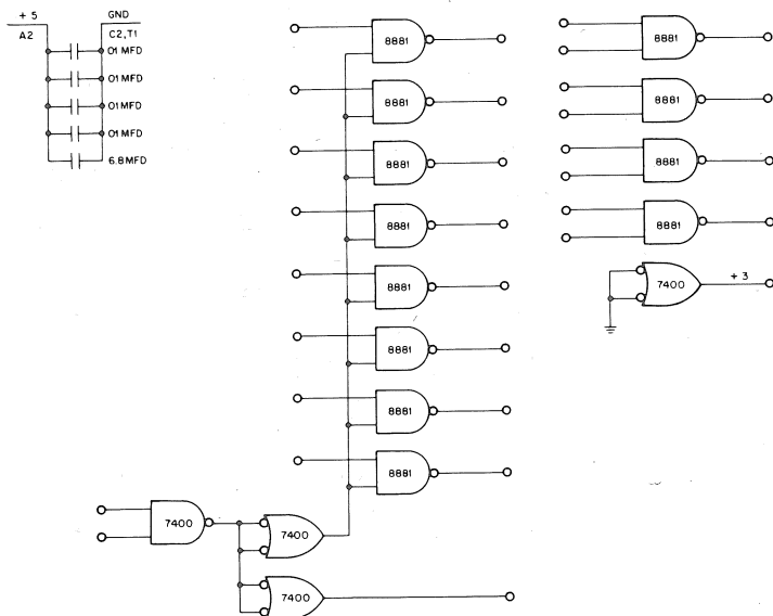
Figure 9.3 M783 Unibus Drivers
