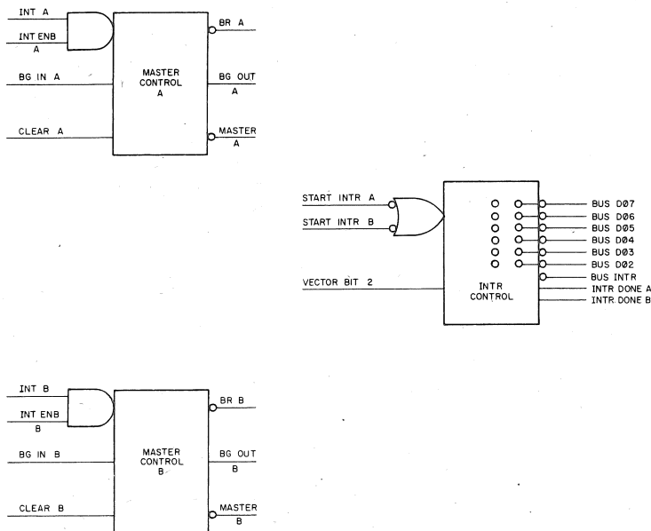
Figure 9.8 M782 Interrupt Control
