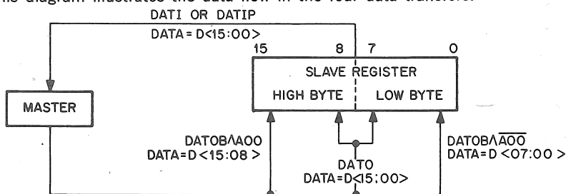
Figure 8-3 Data Flow
