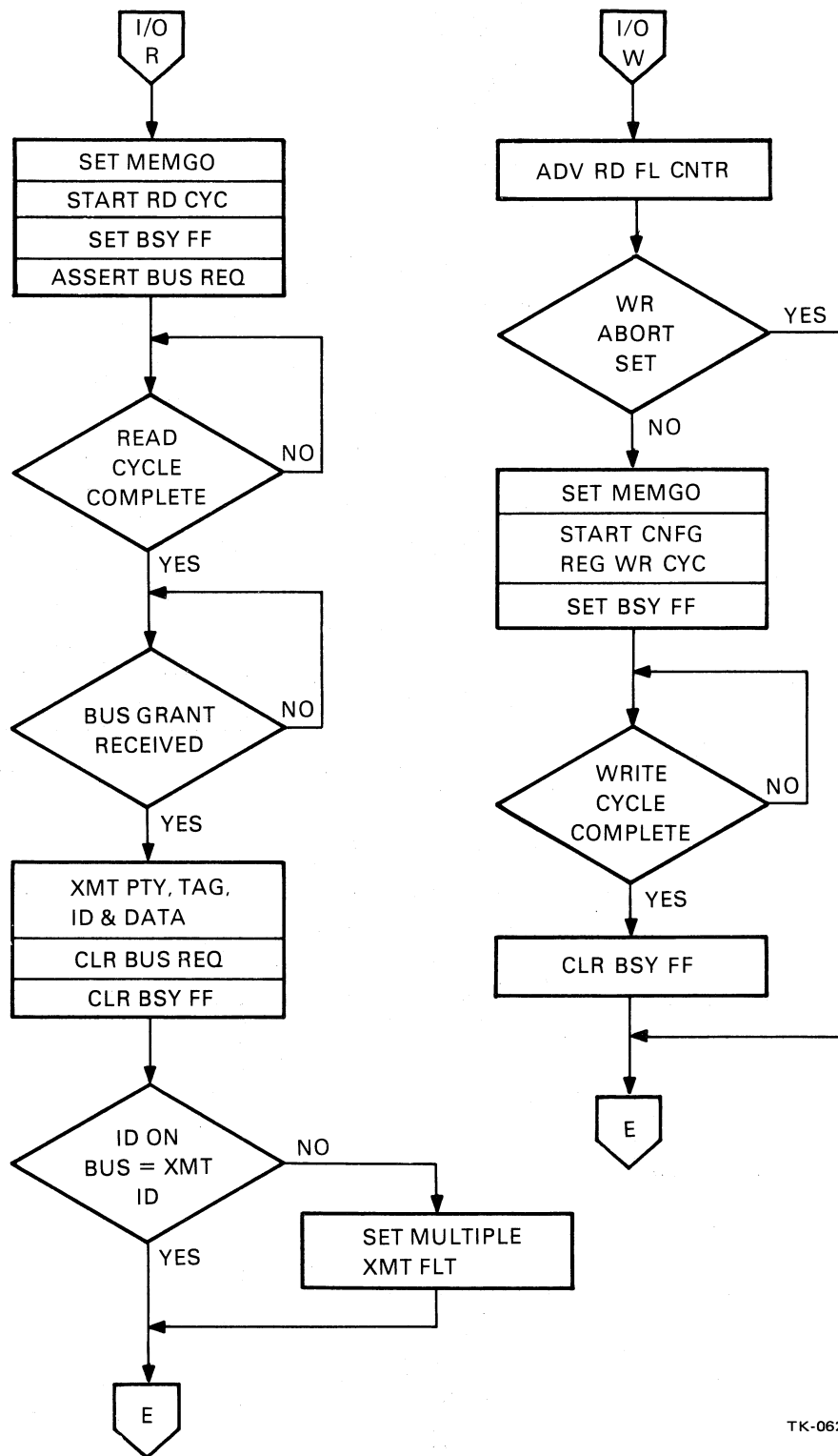
Figure 2-14 I/O Read and Write Cycle Sequences
