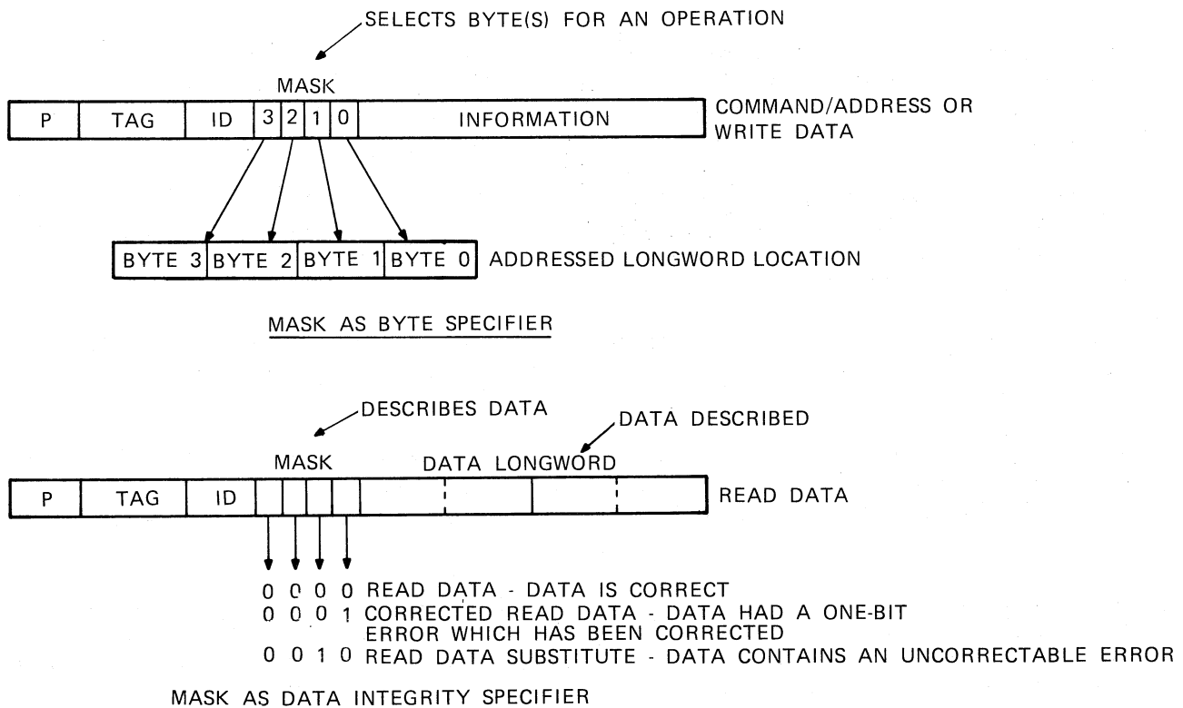
Figure 1-4 Mask Field Interpretation
