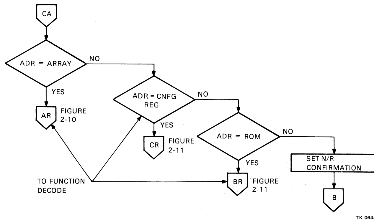
Figure 2-9 Command/Address Destination Decode
