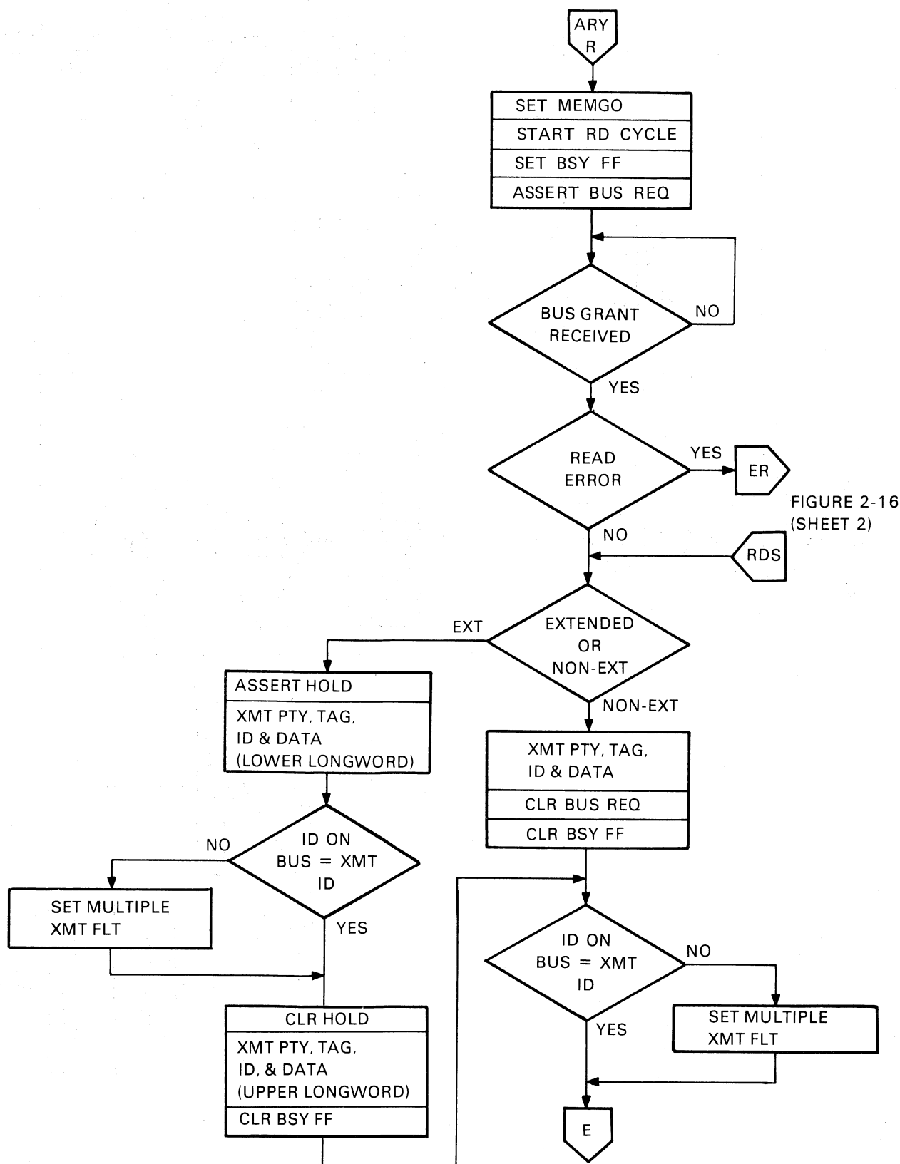
Figure 2-16 Array Read Cycle Sequence (Sheet 1 of 2)
