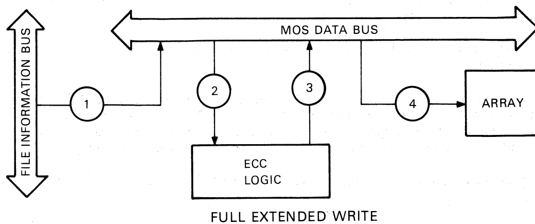
Figure 3-4 Basic Data Flow on the MOS Data Bus
