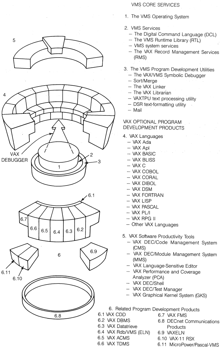
Figure 7-2 ■ The VMS operating system, VAX Languages, VAX Tools, Program Development Utilities, and Related VAX Software Products
