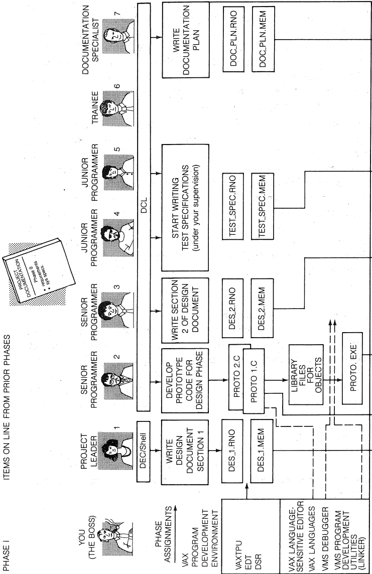
Figure 7-5 ■ Phase 1 — Designing the Software System with VAX/VMS
