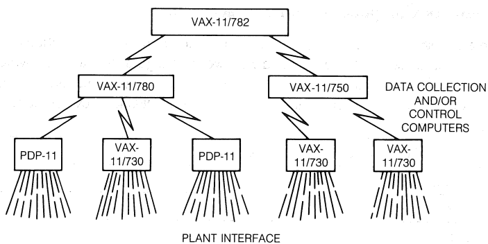
Figure 6-5 ■ Typical Manufacturing Network
