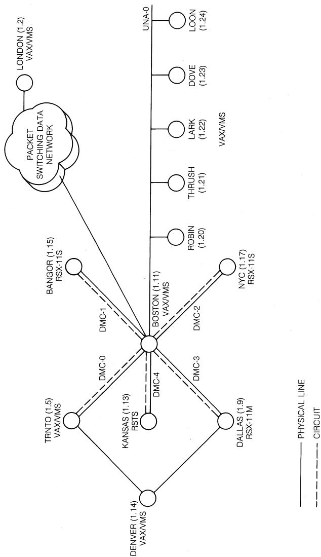
Figure 6-1 ■ Typical Single-Area DECnet Network
