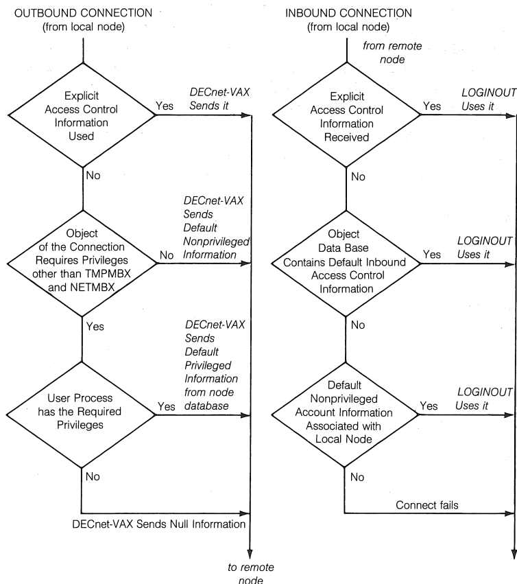
Figure 6-7 ■ Access Control For Inbound Connections
