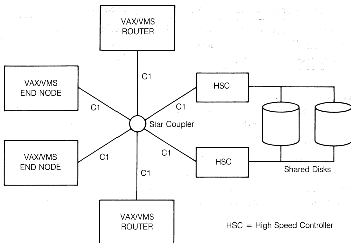
Figure 6-10 ■ A Typical VAXcluster Configuration Using CI As A Data Link
