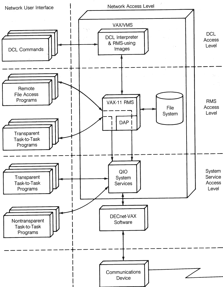
Figure 6-12 ■ Network Access Levels and DECnet-VAX User Interface
