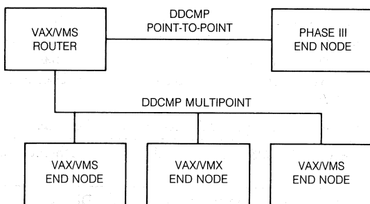
Figure 6-9 ■ Typical DDCMP Point-To-Point Connections
