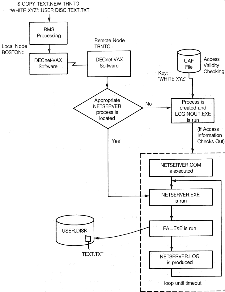
Figure 6-13 ■ Remote File Access Using Access Control String Information
