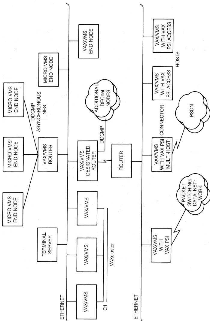
Figure 6-8 ■ Sample DECnet Phase IV Configuration
