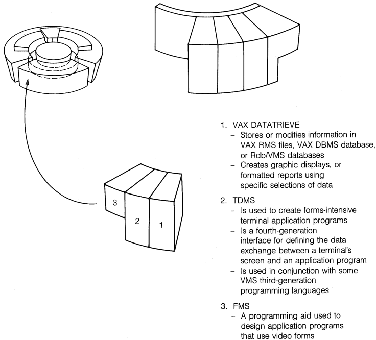
Figure 1-14 ■ VAX Runtime and Forms Management Software Products
