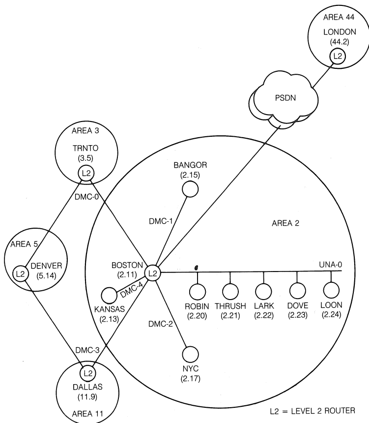
Figure 6-2 ■ Multiple-Area DECnet Network
