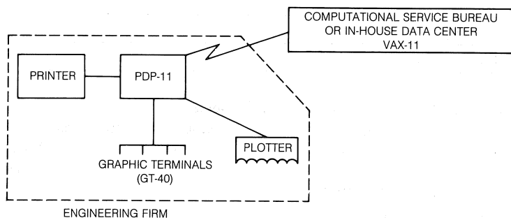
Figure 6-6 ■ Computational Network
