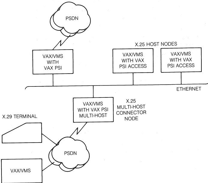
Figure 6-11 ■ DECnet Network Configuration Showing Examples of X.25 Connections
