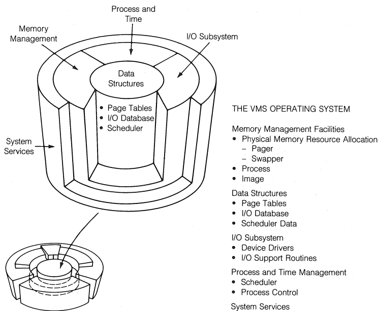
Figure 1-5 ■ The VMS Operating System
