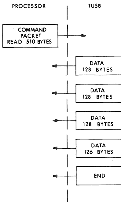
Figure 3-2 READ Command Sequence
