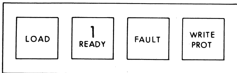
Figure 2-3 RL01/02 FRONT PANEL CONTROLS AND INDICATORS
