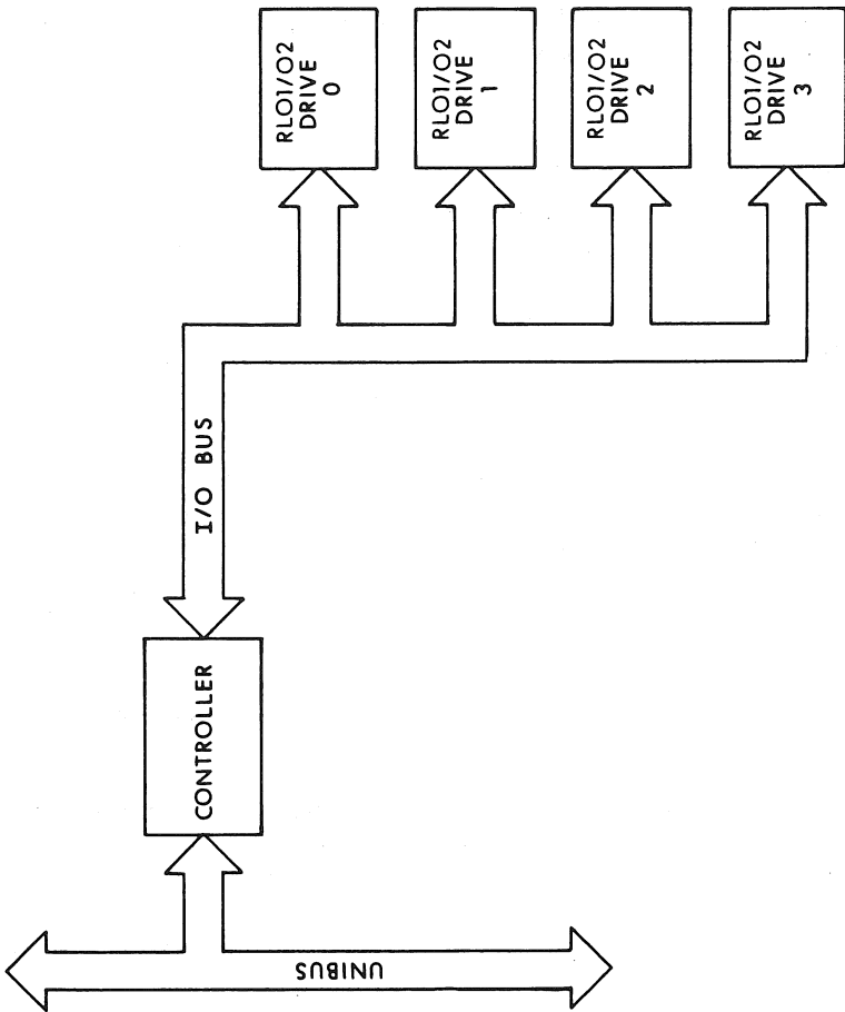
Figure 2-2 RL11/RL211 SYSTEM BLOCK DIAGRAM
