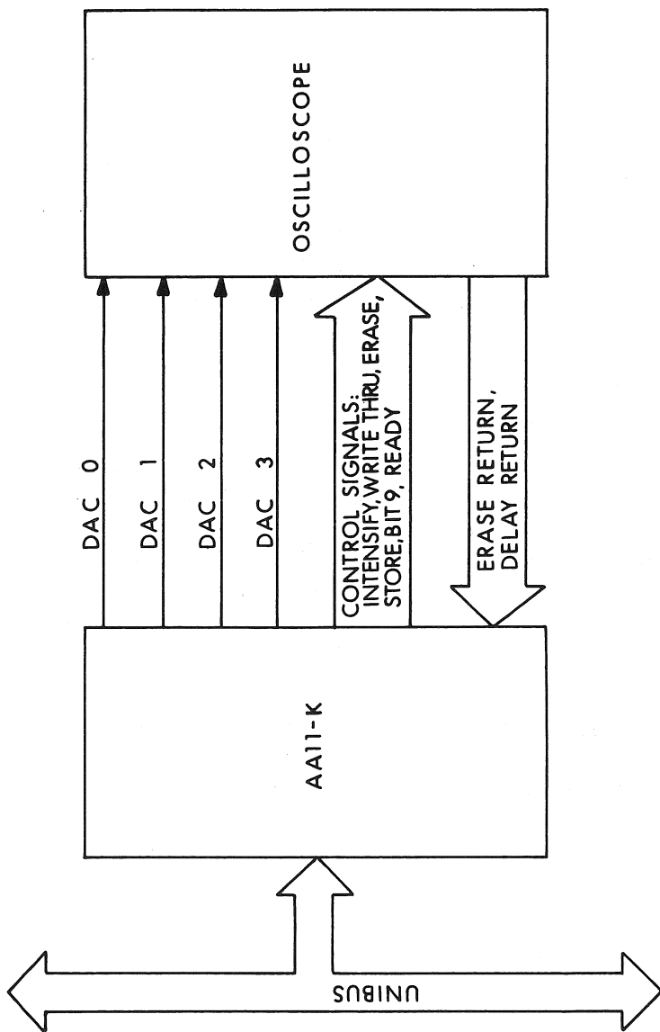
Figure 6-1 AA11-K BLOCK DIAGRAM
