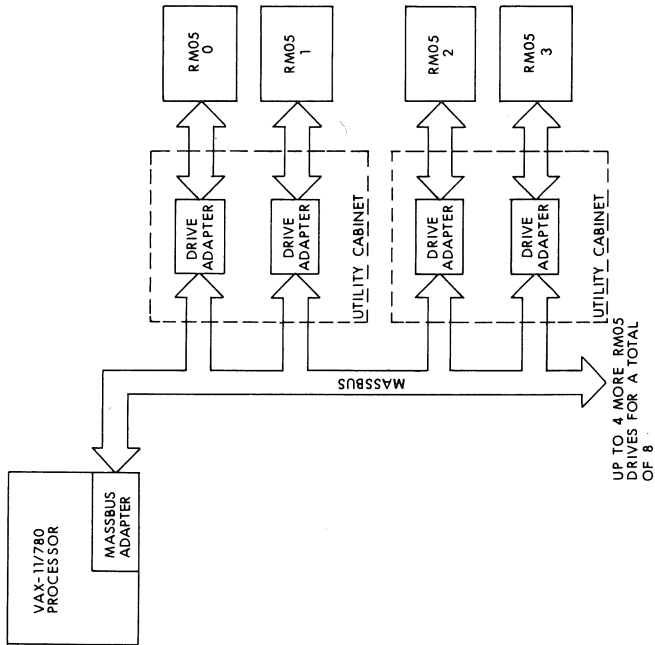
Figure 2-17 REM05 SYSTEM BLOCK DIAGRAM
