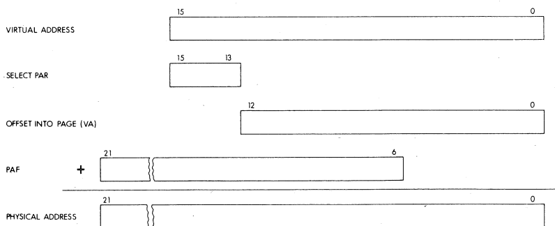
Figure 6-9 Construction of a Physical Address
