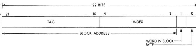
Figure 7-5 Physical Address
