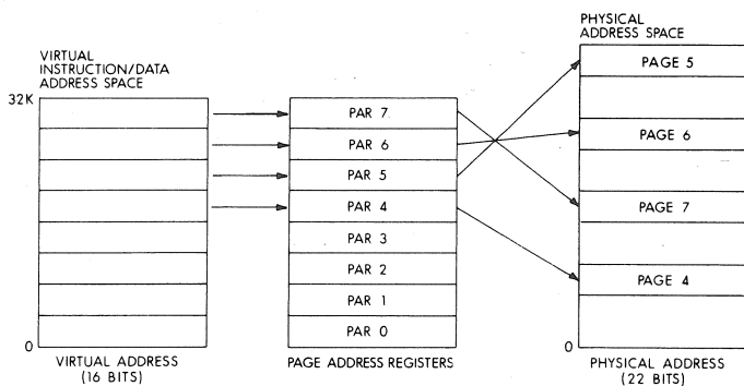
Figure 6-6 Virtual Address Mapping into Physical Address
