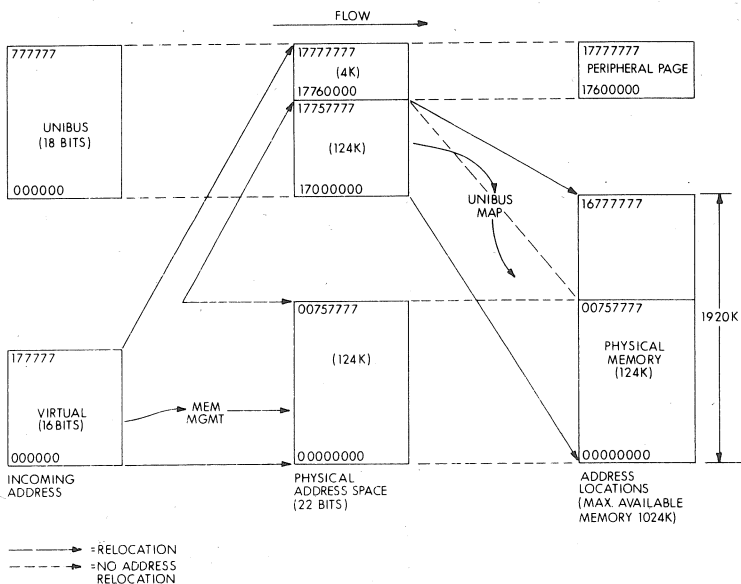
Figure 6-4 18-Bit Mapping
