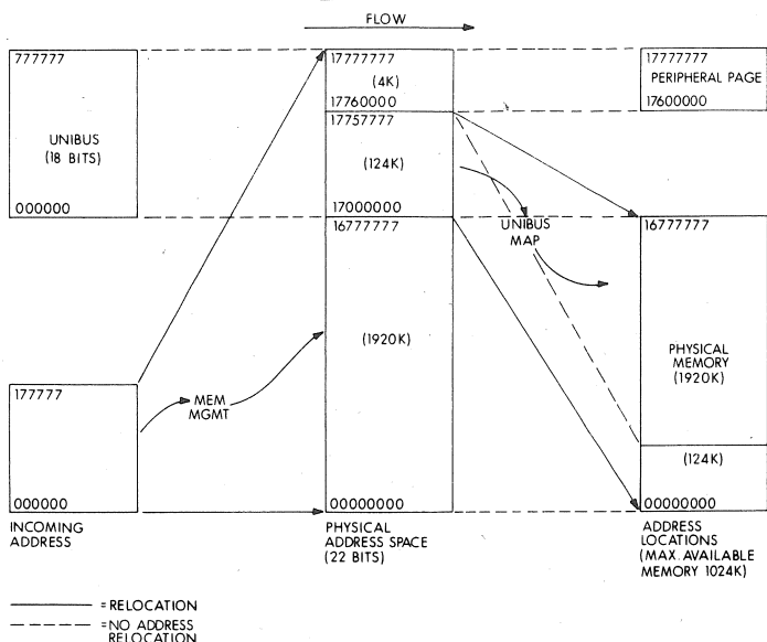
Figure 6-5 22 Bit Mapping
