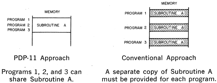
Figure 9-15: Reentrant Routines
