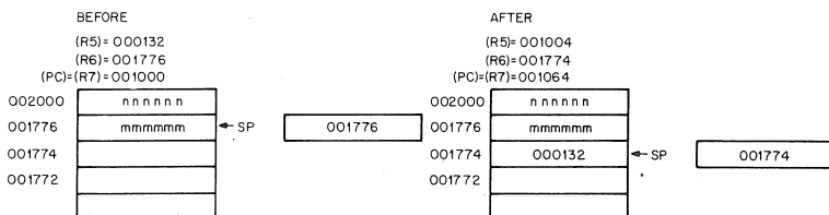
Figure 9-8: JSR
