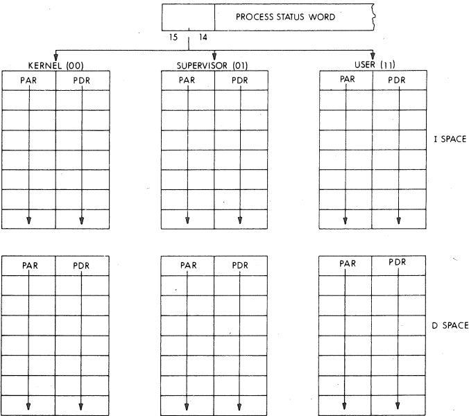
Figure 6-10 Active Page Registers
