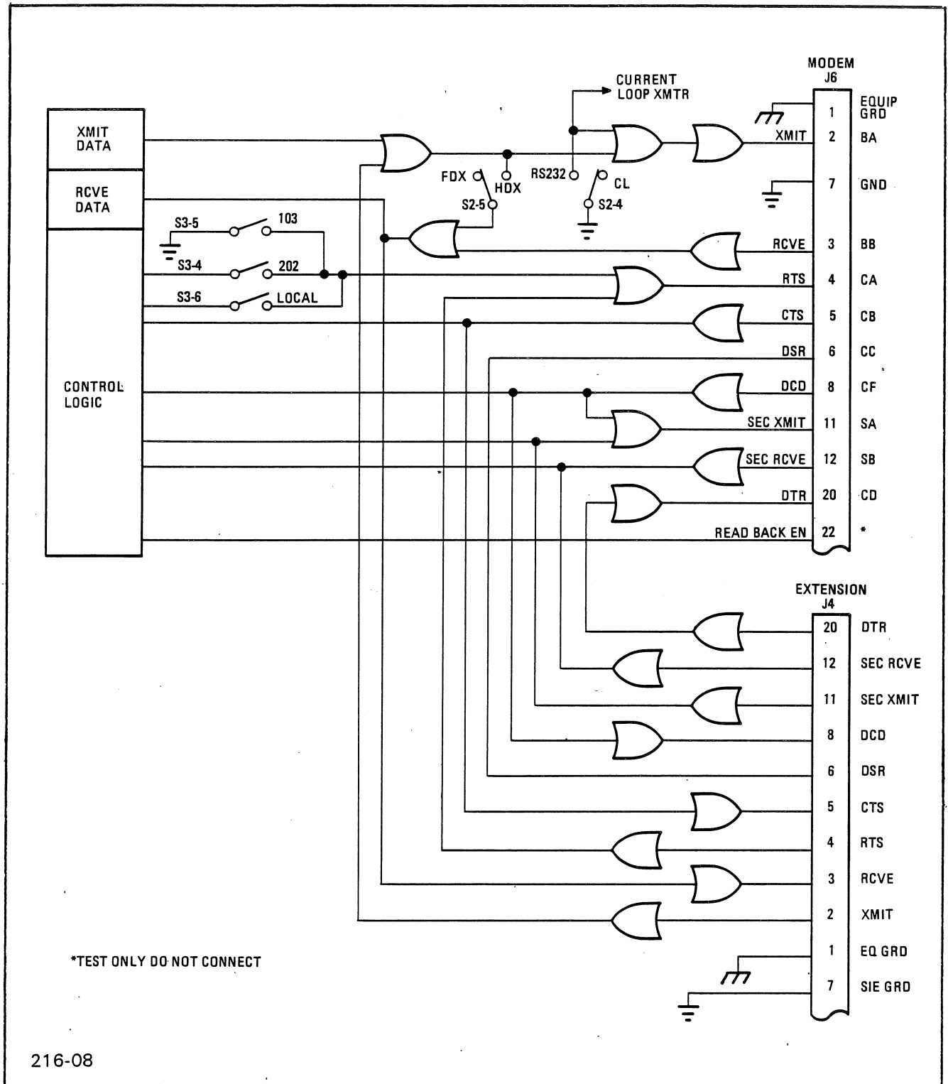
Figure 2-3. RS-232C MODEM and EXTENSION Interface Logic
