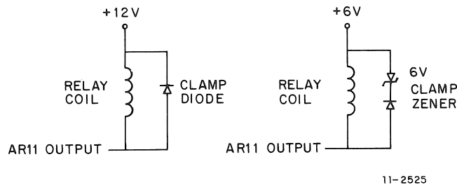
Figure 4-3 Clamping Circuits for Inductive Loads
