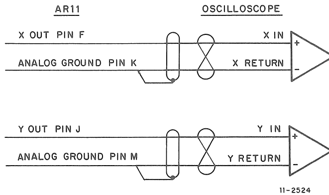
Figure 4-2 Connection to Oscilloscope with Differential Input
