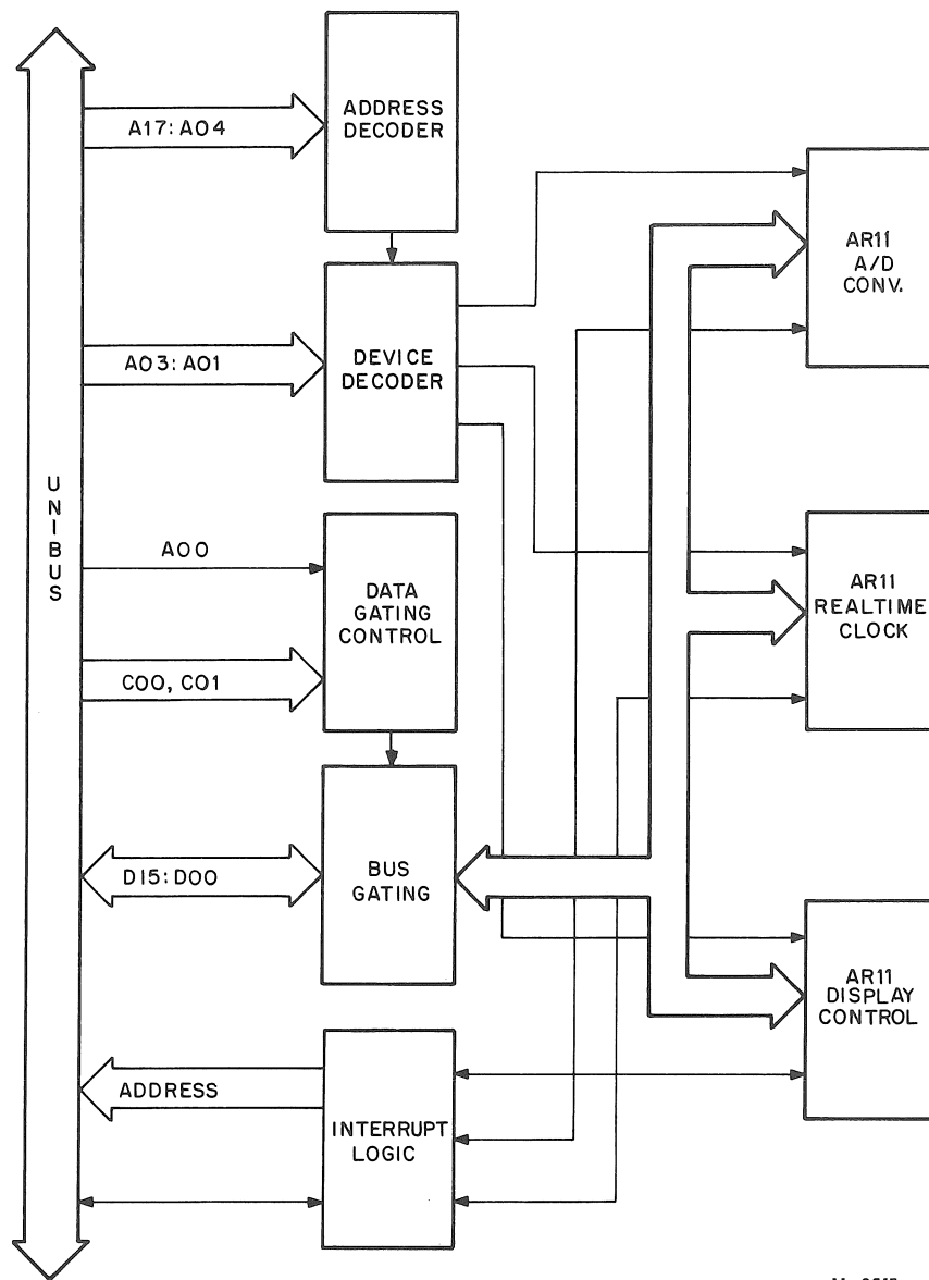
Figure 1-1 AR11 Block Diagram
