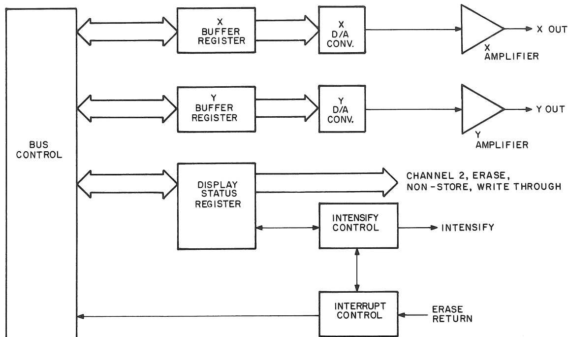
Figure 4-1 Display Control Block Diagram
