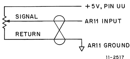
Figure 2-3 Use of +5 V Supply Output
