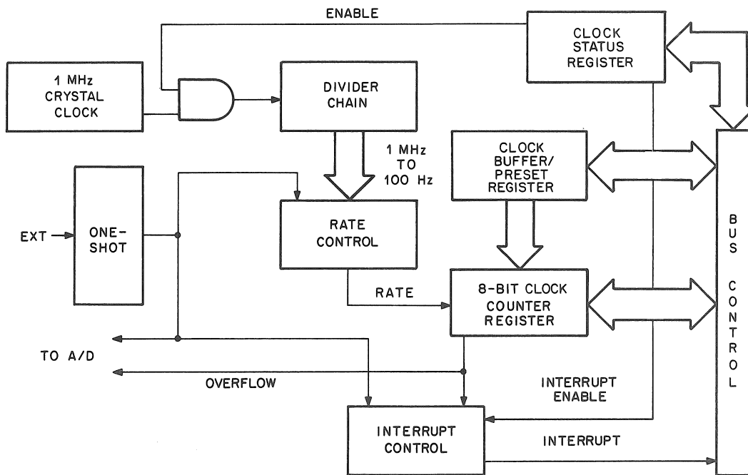
Figure 3-1 Clock Block Diagram
