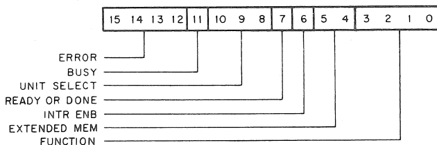
Figure 1-13 Preferred CSR Bit Assignments
