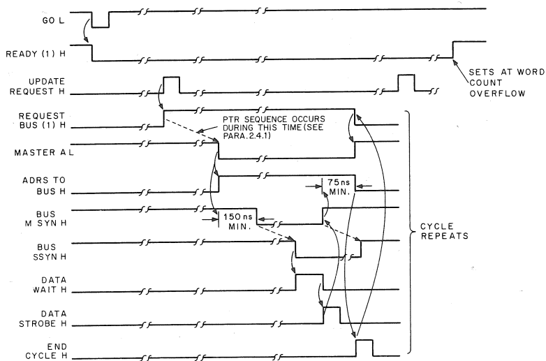
Figure 3-11 DAC-DMA Interface (timing diagram)
