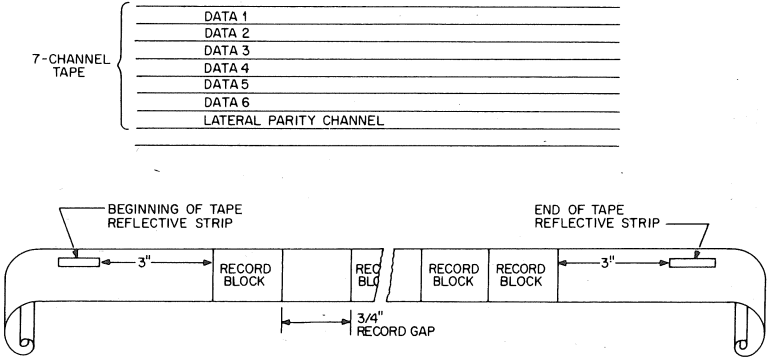
Figure 3-3 - Magtape Format
