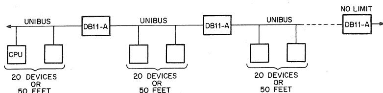
Figure 7-1 DB11 Bus Repeater
