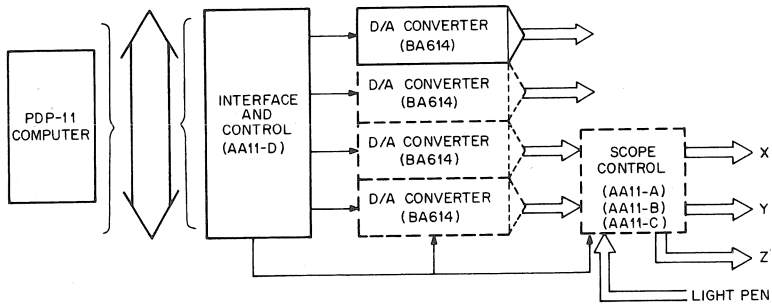
Figure 9-2 - AA11-D Subsystem
