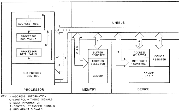
Figure 1-1 PDP-11 Interface Block Diagram
