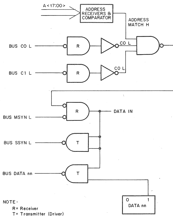
Figure 1-12 Slave Logic for DATI (Fast Response)
