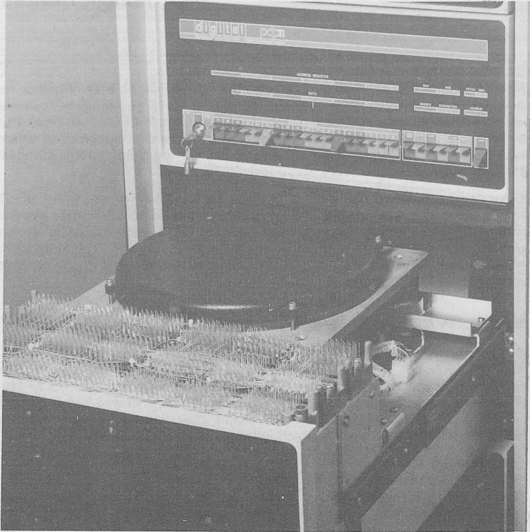
RC11/RS64 DECdisk
