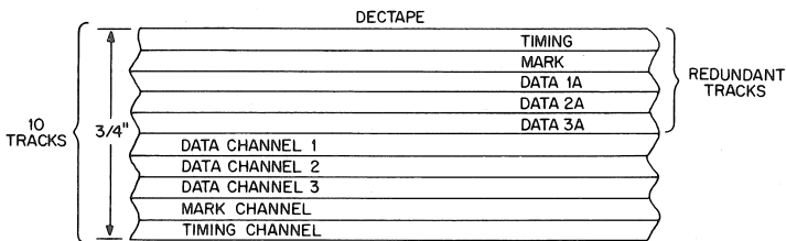
Figure 3-1 - DECTape Format
