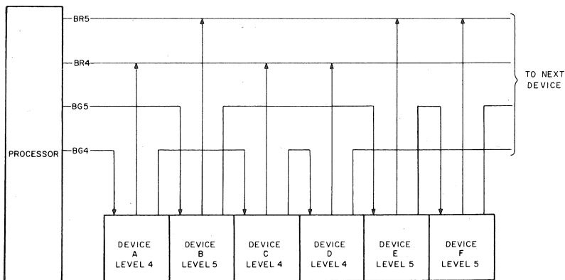
Figure 1-8 Priority Chaining Example
