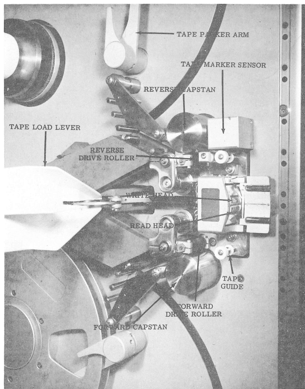
Figure 5. Tape Handler Mechanism Parts
