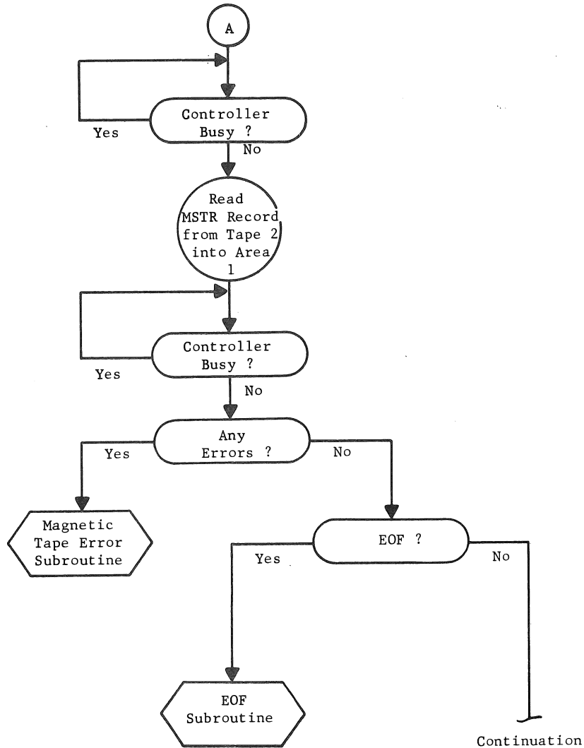
Flow Chart 2
