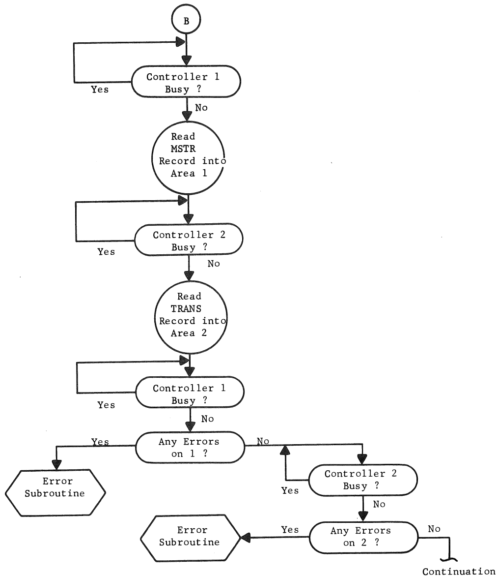
Flow Chart 3
