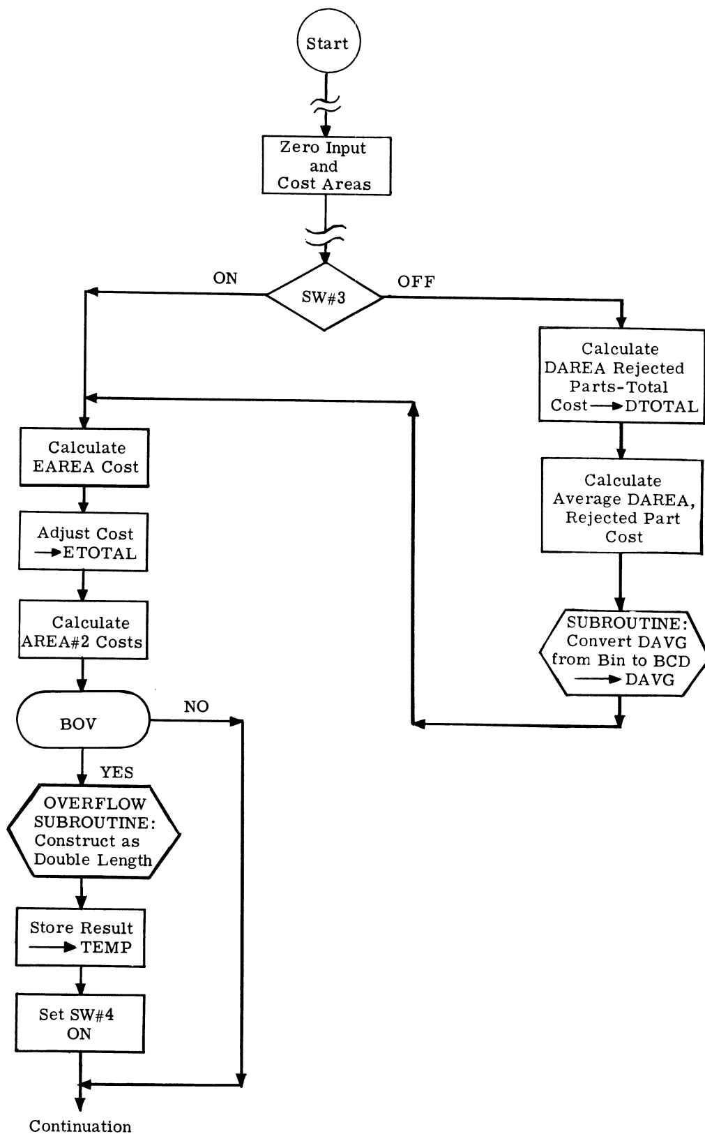
Figure 5-7. Rejected Parts Cost Flow Chart
