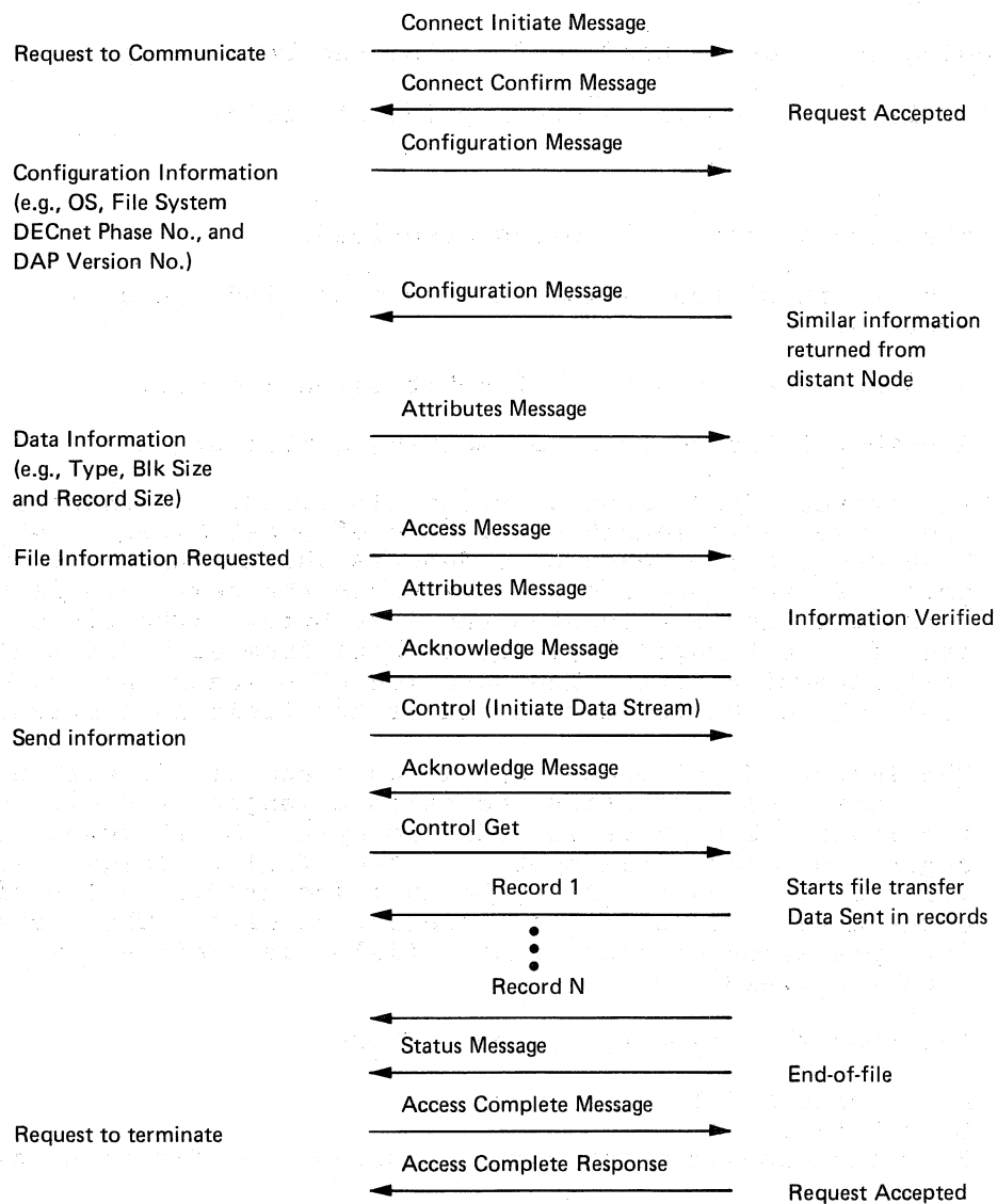
Figure 2-1. Typical DAP Message Exchange (Sequential File Retrieval)
