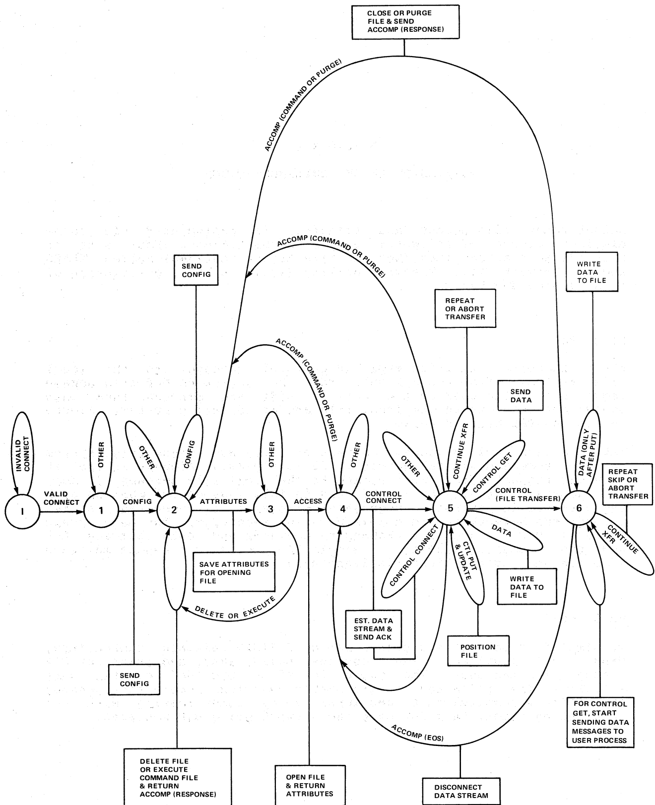
Figure B-1. FAL State Diagram
