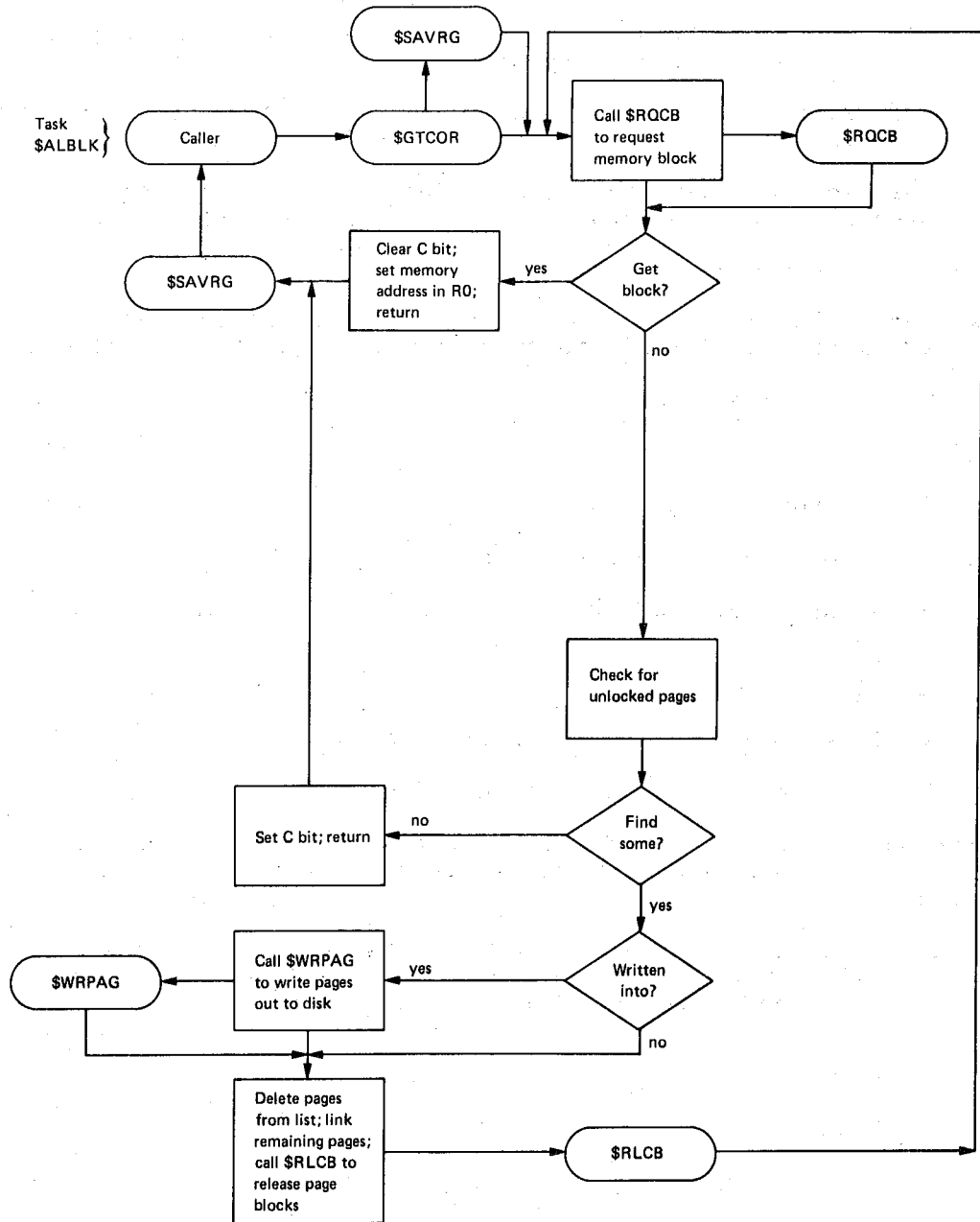
Figure 8-3A General Block Diagram of the $GTCOR Routine (nonstatistical module GTCOR)
