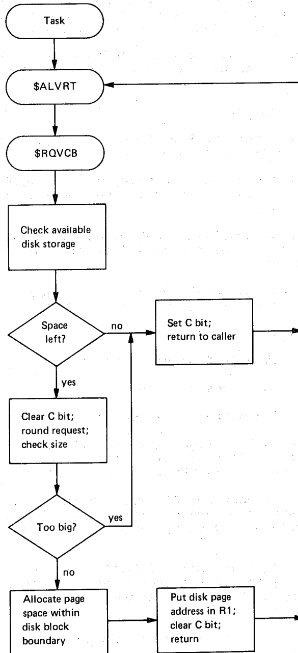
Figure 8-8 General Block Diagram of the $RQVCB Routine
