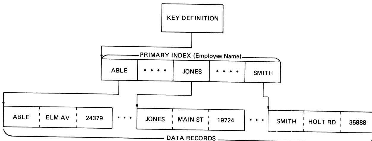
Figure 6-3 Indexed File Organization
