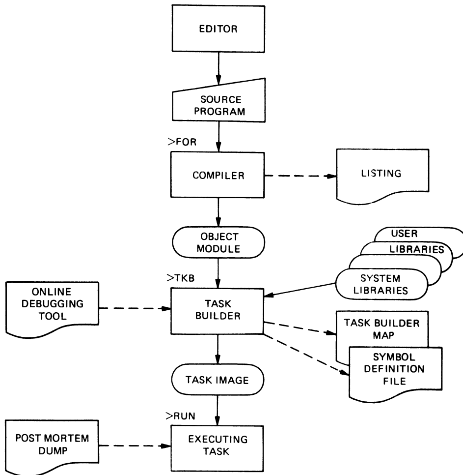
Figure 5-1 Steps to Creating a FORTRAN Program
